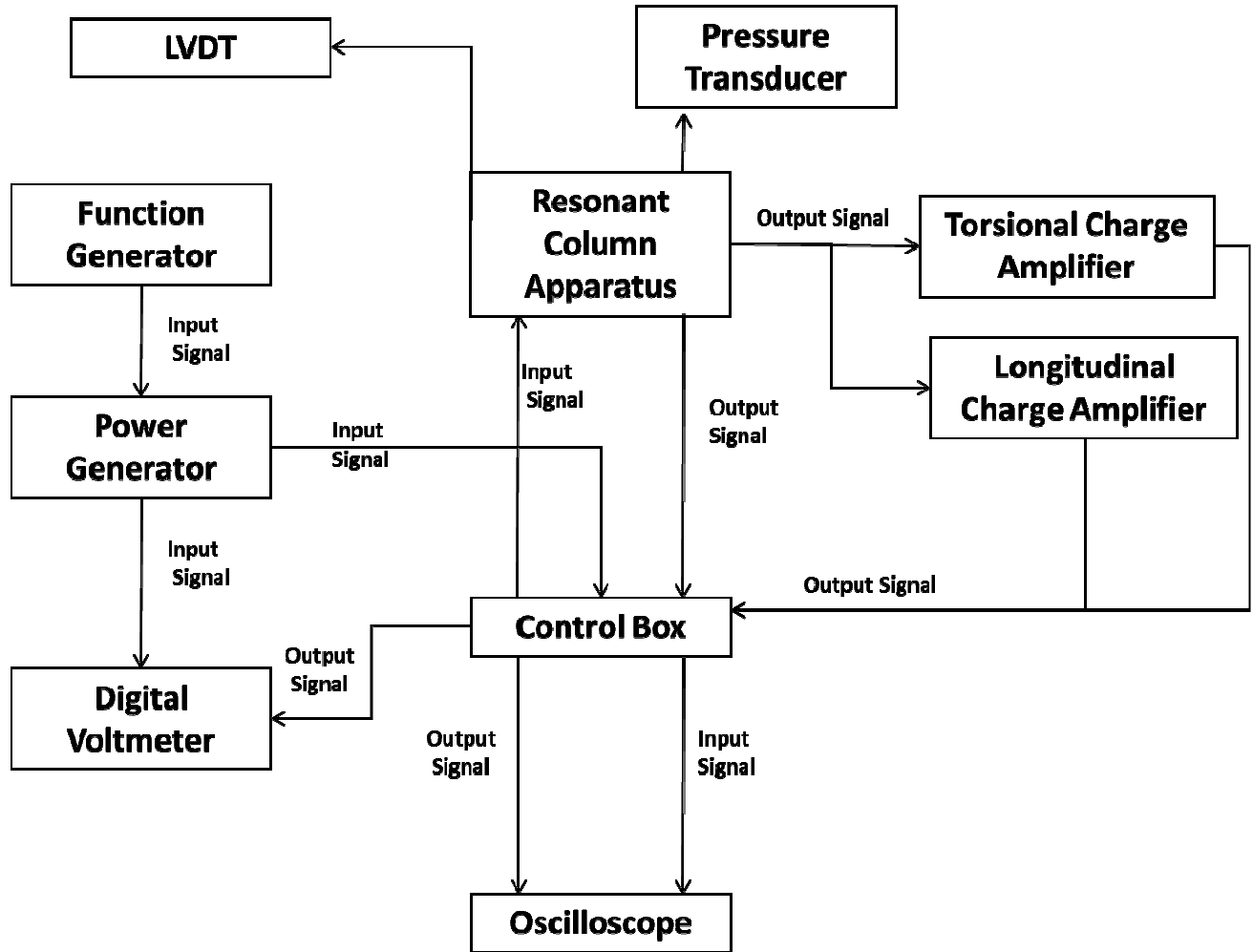
Figure 3.7-Consolidated Wiring Schematic
