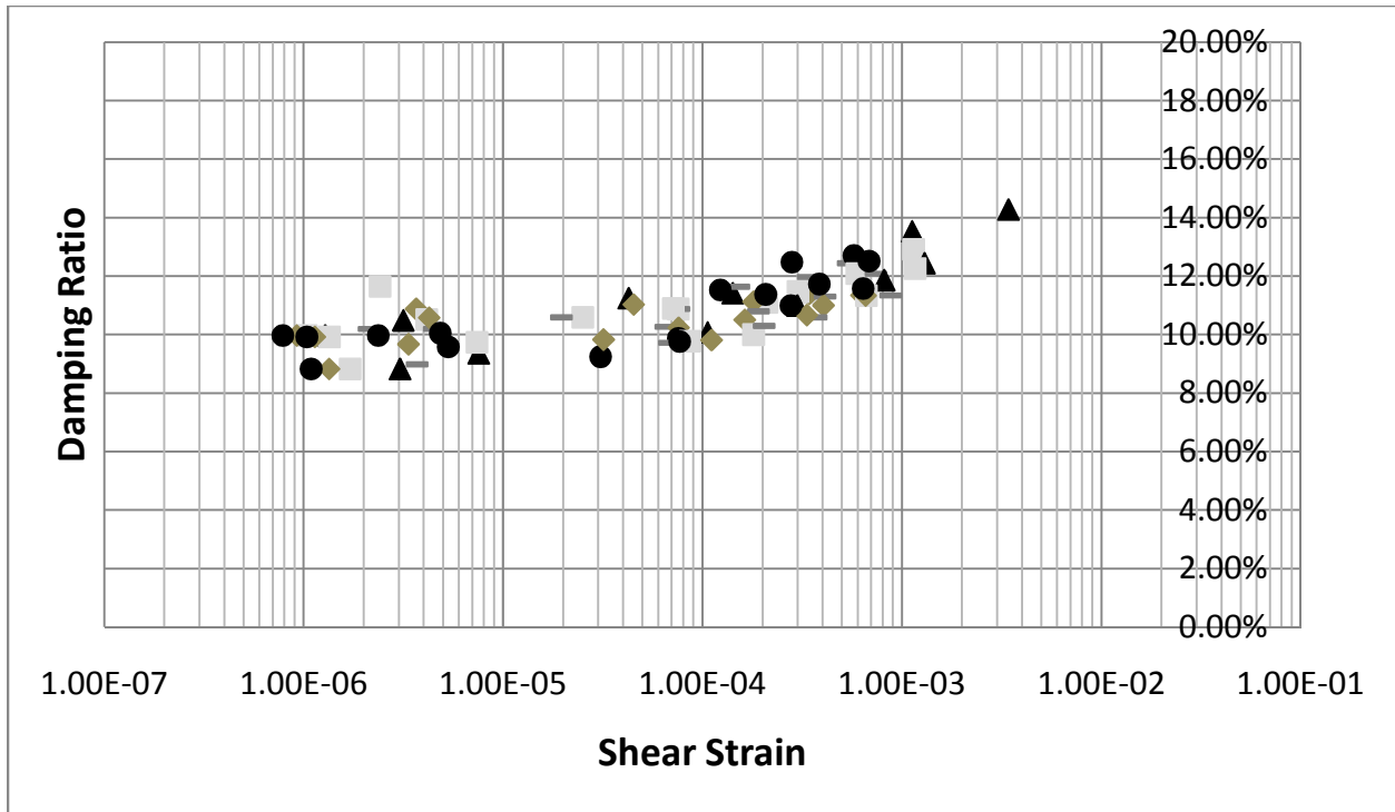
Figure 5.12- Damping Ratio for Remolded Heated
