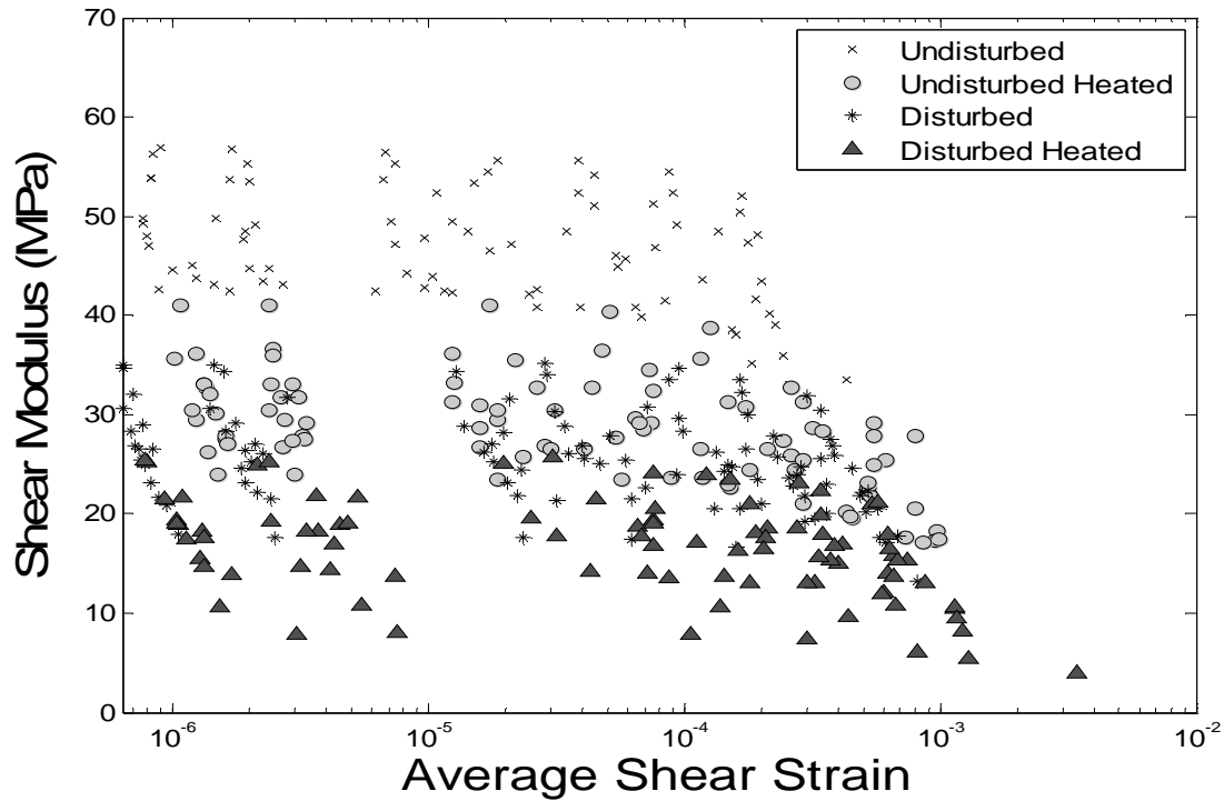
Figure 5.3- Shear Modulus by Preparation Method
