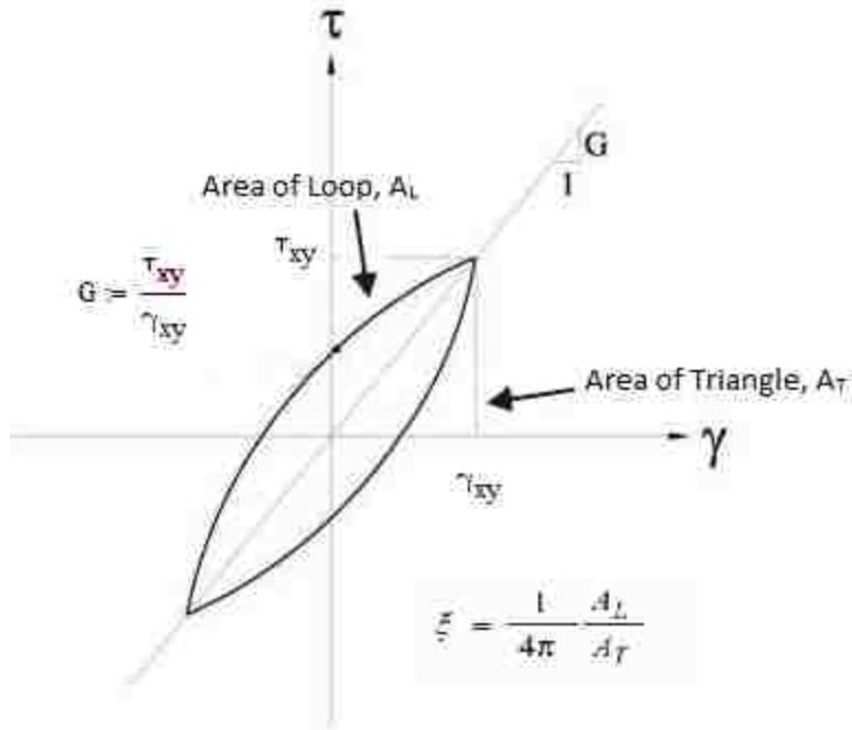
Figure 2.1-Hysteresis Loop
